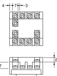
端子配置 (BOTTOM VIEW)
